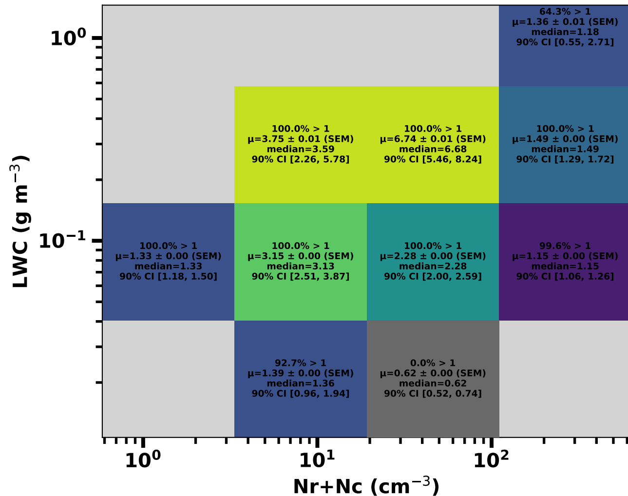
CAS RWC GCCN Concentration
