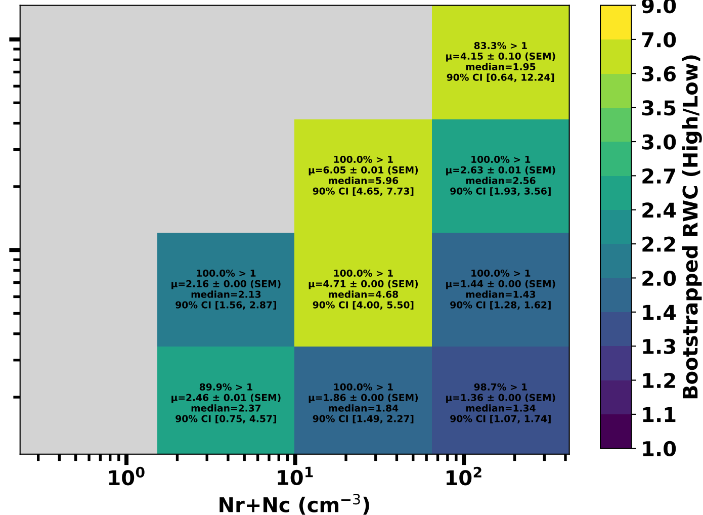
CDP RWC GCCN Concentration
